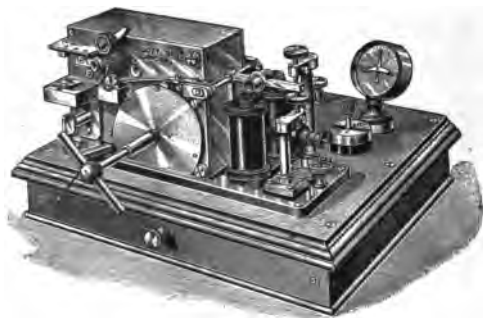
FIG. 49.—Morse Inkwriter.
